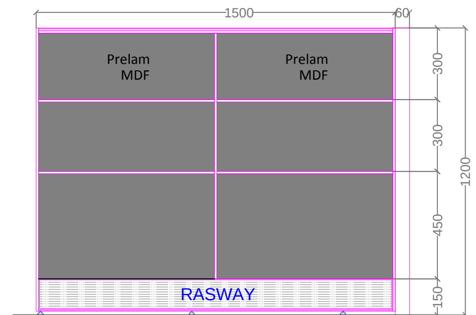
ELEVATION_B Out Side Elevation
