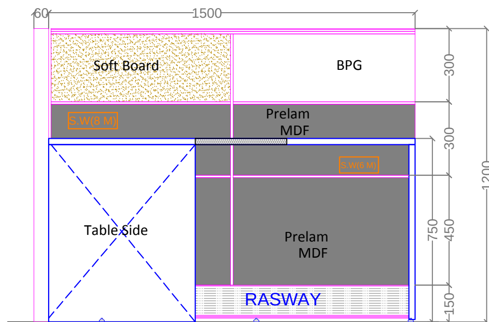
ELEVATION_B In Side Elevation (60 mm LOW HEIGHT PARTITION)
