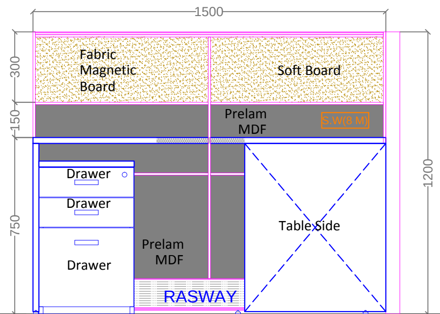
ELEVATION_A in Side Elevation
